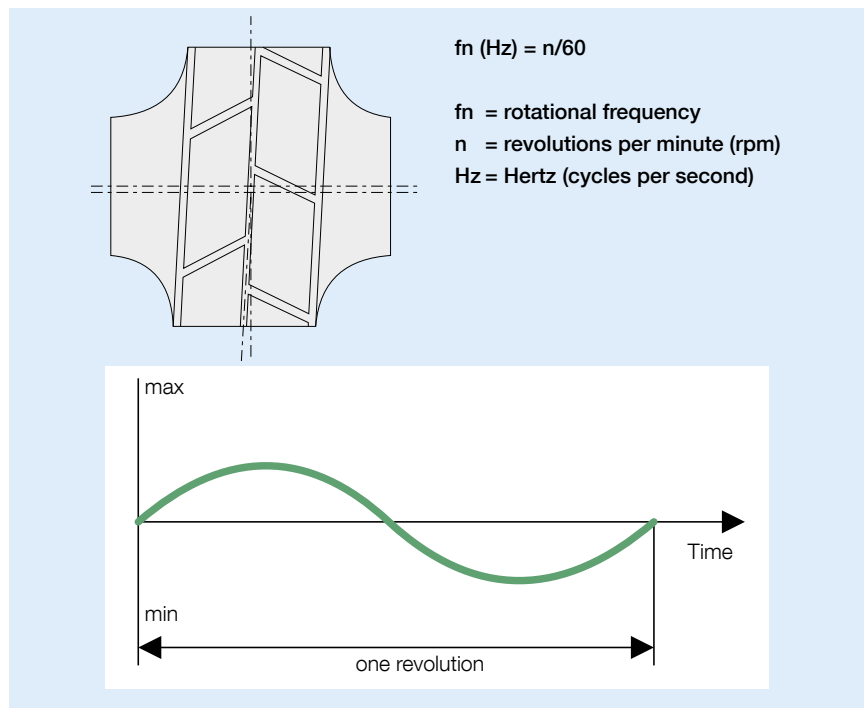
Fig. 7. Pressure pulsations at rotational frequencies
