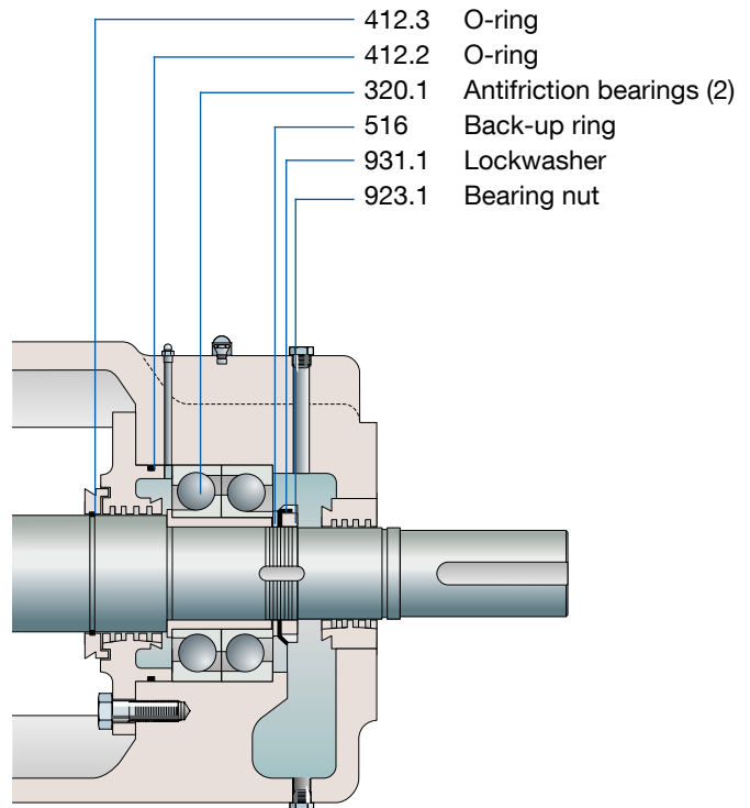
Bearing Unit Service Kit for HPP Pumps
