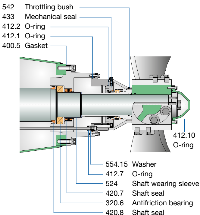
Shaft Seal Service Kit for SLG/SLB Agitators with Single Mechanical Seal with Labyrinth and Flushing
