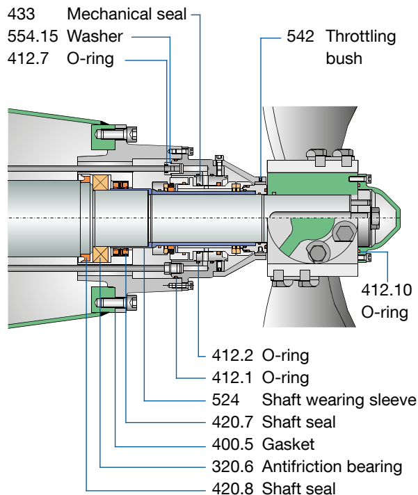
Shaft Seal Service Kit for SLF Agitators with Double Mechanical Seal
