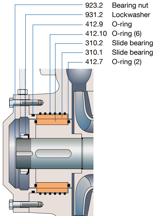
Balancing Drum Service Kit for HPP Pumps
