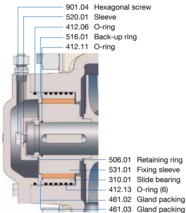
Balancing Drum Service Kit for MBN Pumps
