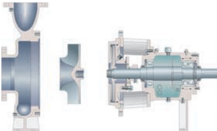
Existing casing and impeller
